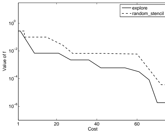
Figure 3.2. Iteration History with Random Exploration
