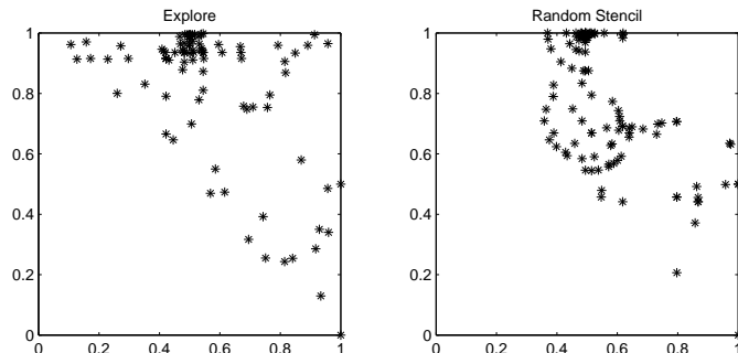
Figure 3.3. Complete History with Random Exploration
