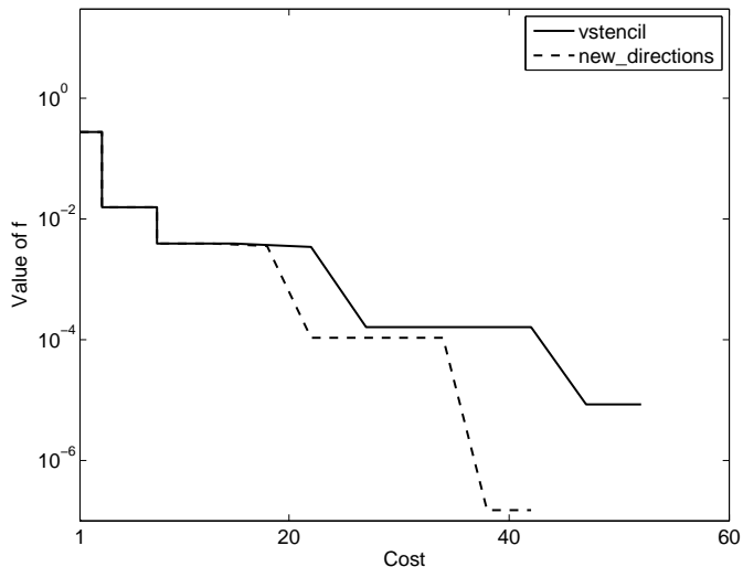
Figure 3.1. Iteration History with Extra Directions
