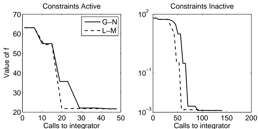
Figure 4.6. Levenberg-Marquardt Executive Results
