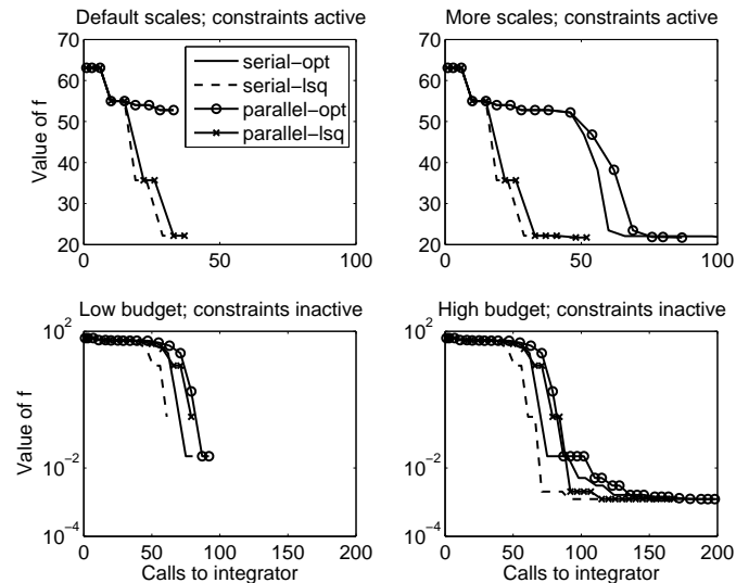
Figure 4.2. Optimization History: Parameter ID Revisited
