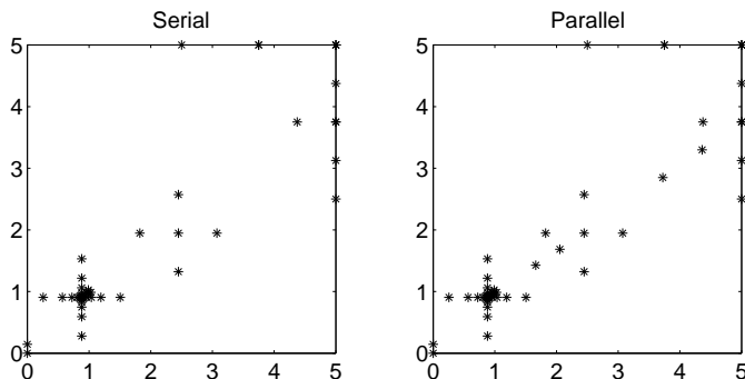
Figure 4.3. Where is the function evaluated?
