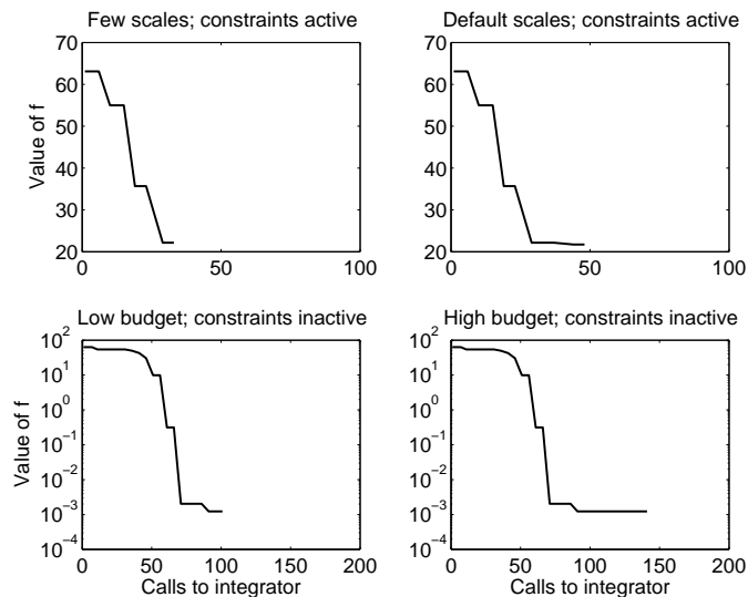
Figure 4.1. Iteration History: Parameter ID
