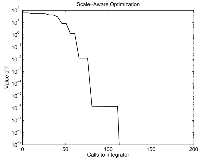
Figure 4.4. A Scale-Aware Function
