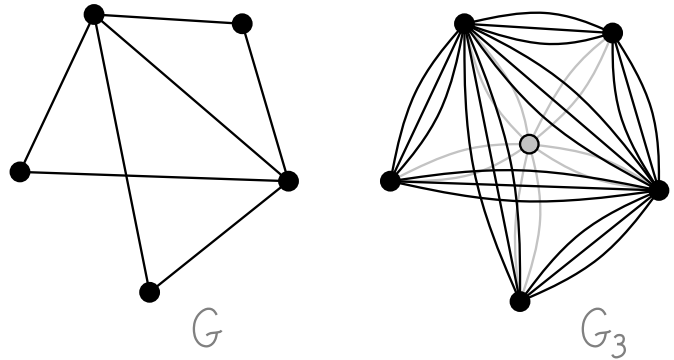
Figure 1: Reducing EULERIAN ORIENTATION COUNT TO ORB COUNT
